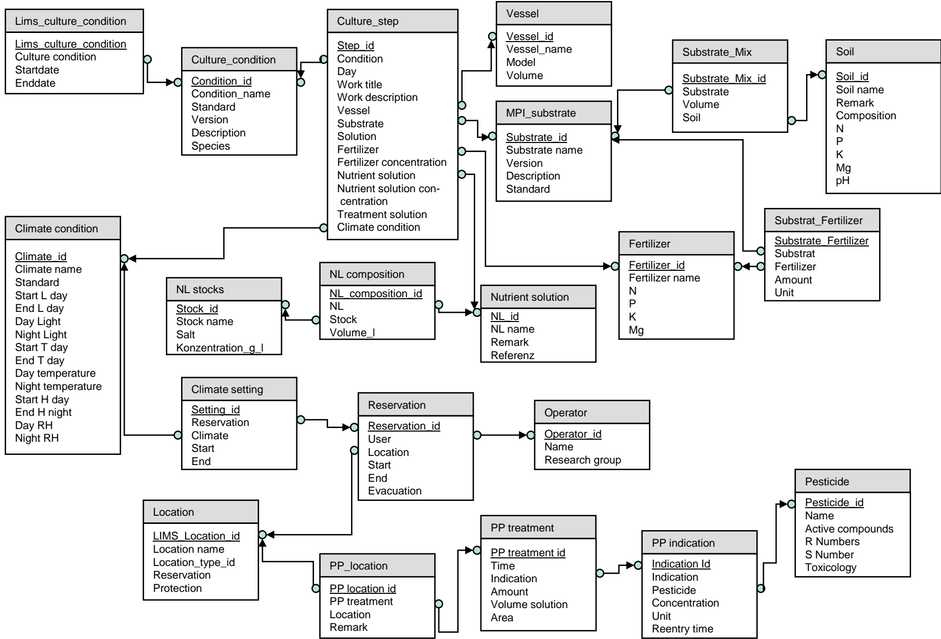
Diagram displaying the entity-relationship-model of the ACCESS database used by the plant cultivation service. Upper half displays tables to describe standard cultivation protocols and their link to the LIMS system. In this part, the cultivation steps and the containers, substrates, fertilizers and nutrient solutions used in these steps are documented. The lower half shows tables containing information on locations like reservation status and climate conditions in plant cultivation sites (locations) and pesticides that have been applied in these locations. Objects are depicted as rectangles containing the respective attributes, foreign key relations as arrows. Primary key attributes are underlined.
